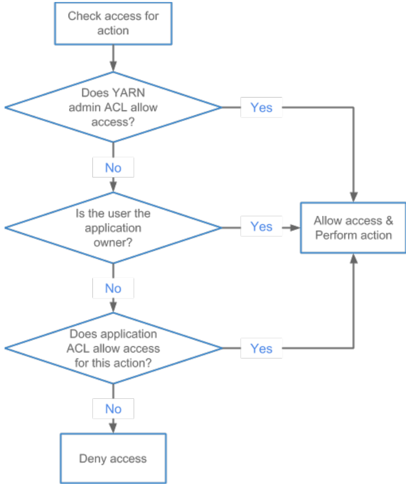
Figure 2: Application ACL Evaluation Flow
